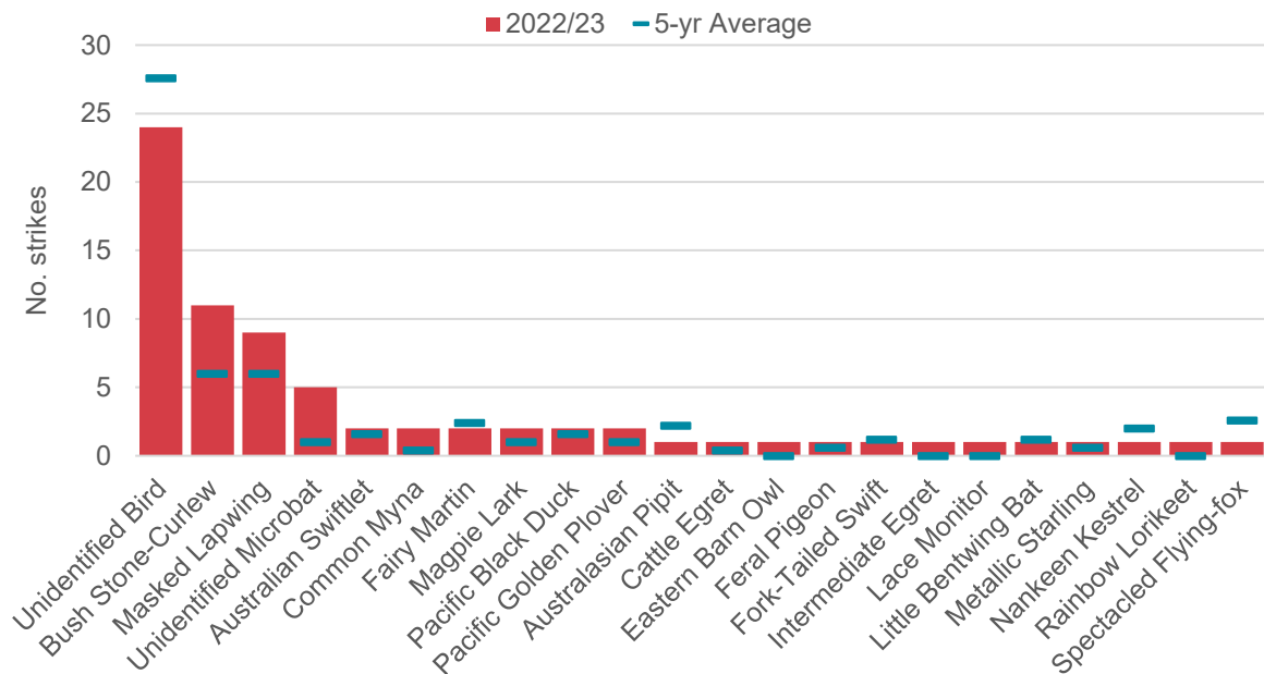
Figure 8. Total confirmed on-airport and airport vicinity species struck versus 5-year average, CNS, 2017/18-2022/23.
